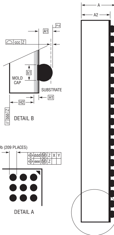
DETAIL B PACKAGE SIDE VIEW
